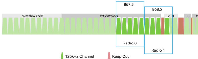
Figure 35: Channel plan graphic
