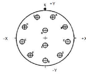
Contact Layout
