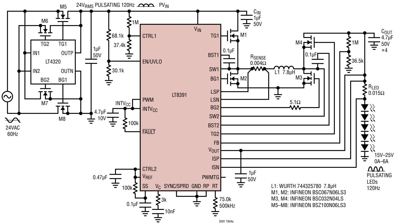
98% Power Factor from 60Hz 24VAC Input
