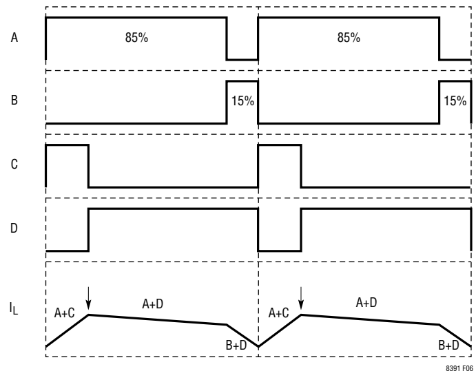
Figure 6. Peak-Boost in Buck-Boost Region ( V_{IN} \lesssim V_{OUT} )
