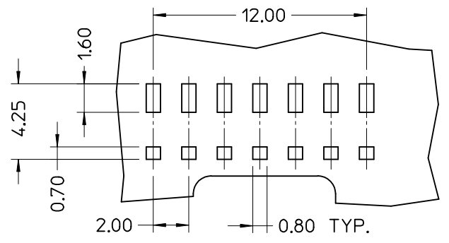
RECOMMENDED PCB LAYOUT (VIEW FROM COMPONENT SIDE) SCALE 5:1
