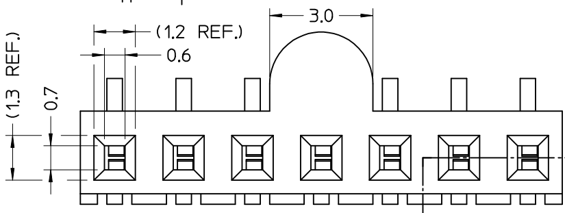
SECTION G-G
