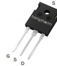
TP65H035G4WS TO-247 (top view)
