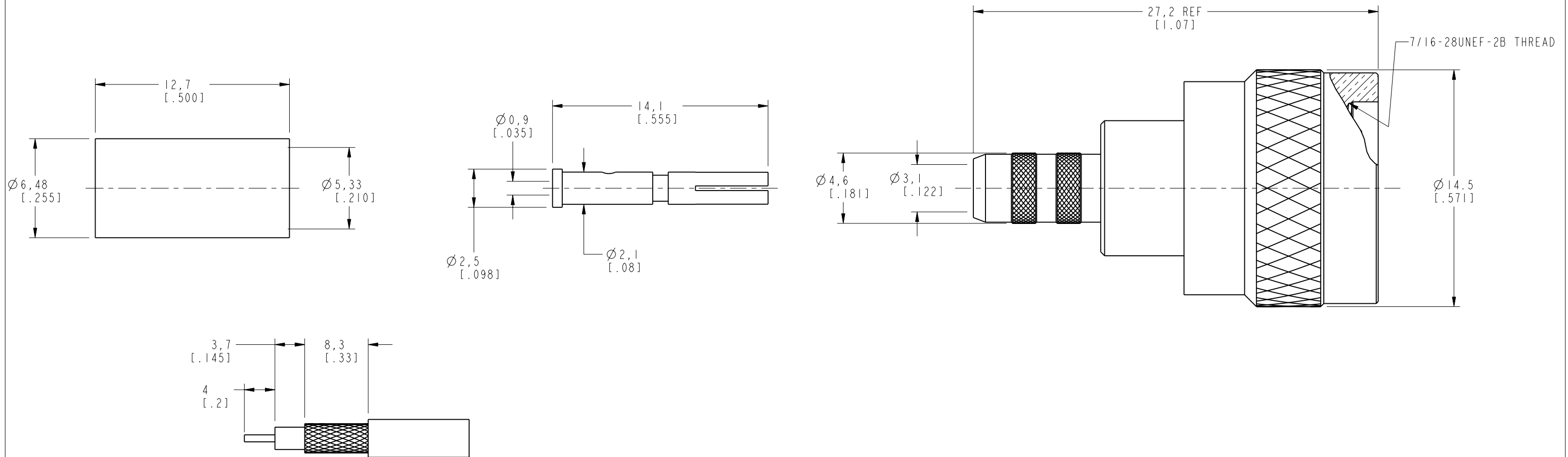
RECOMMENDED CABLE STRIPPING DIMENSIONS SCALE 2.000
