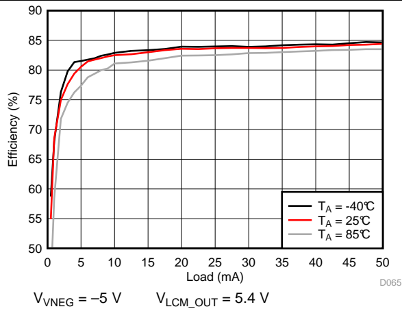
Figure 86. VNEG Efficiency
