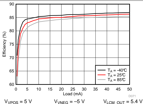
Figure 92. VPOS/VNEG Efficiency
