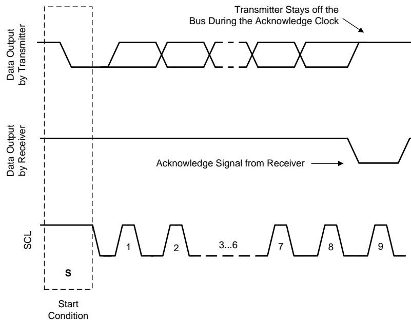
Figure 34. Acknowledge Signal
