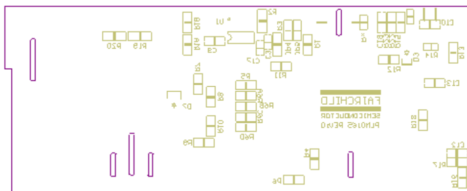
Figure 36. Bottom Assembly
