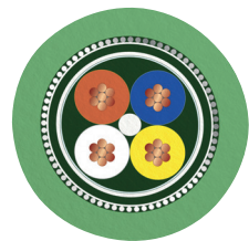
PROFINET stranded CAT5 [93M]
