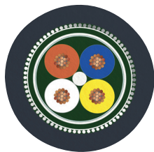
PROFINET RADOX® railway application CAT5 [937]
