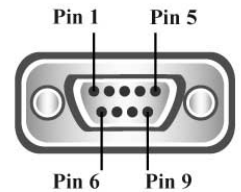
RS422/485 Pinout (9 Pin)
