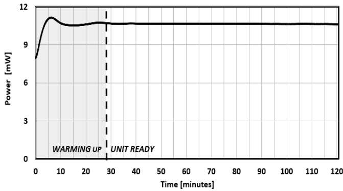
FIG. 7: WARM-UP TIME
