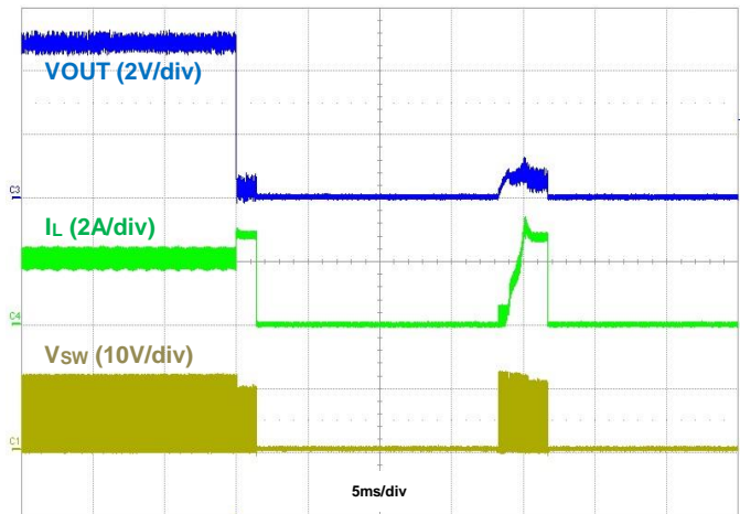
Figure 13. Output Short Protection, IOU = 2A
