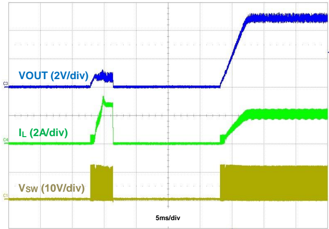
Figure 14. Output Short Recovery, IOU = 2A
