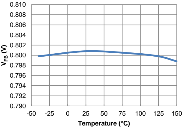
Figure 15. Feedback Voltage vs. Temperature, IOU = 1A
