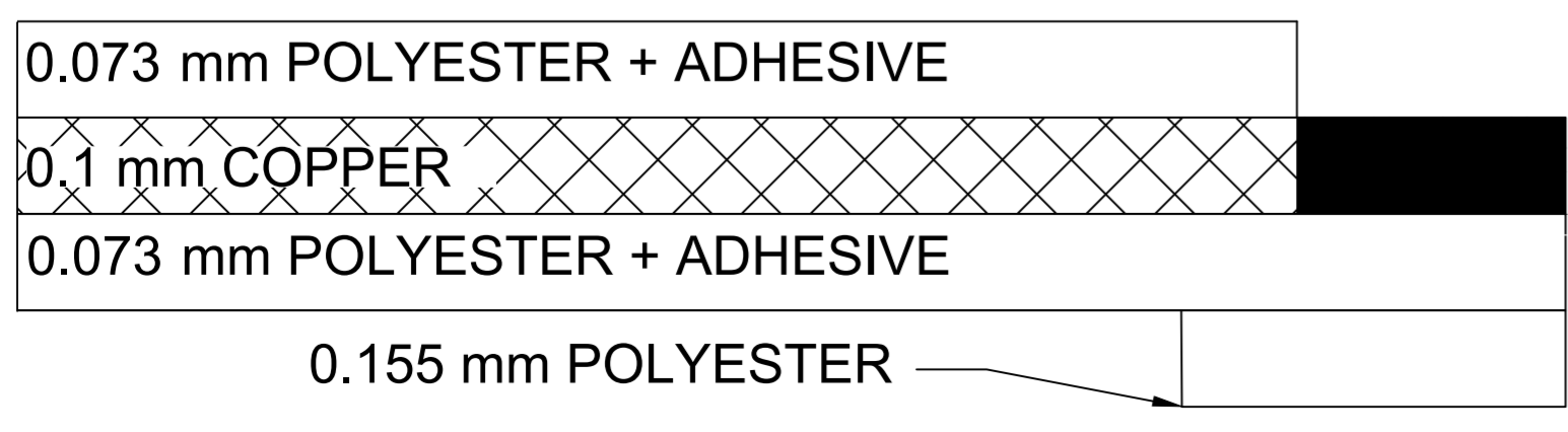
CROSS-SECTION
