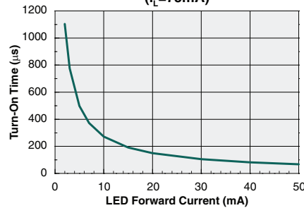
Typical Turn-On vs. LED Forward Current ( I_L=75mA )
