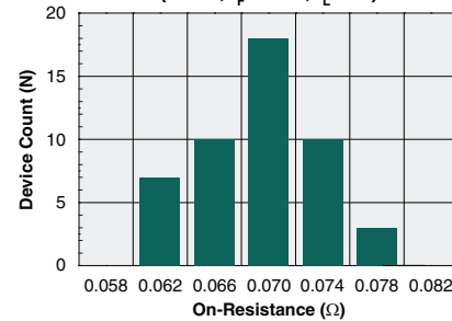
Typical On-Resistance Distribution (N=50, I_F=5mA , I_L=1A )
