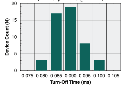
Typical Turn-Off Time (N=50, I_F=5mA , I_L=75mA )
