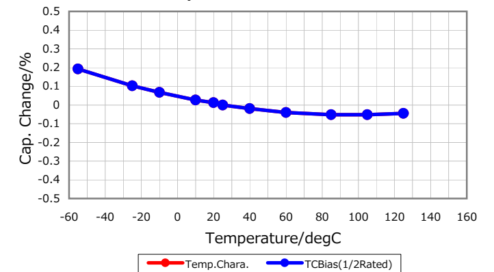
Temperature Characteristics
