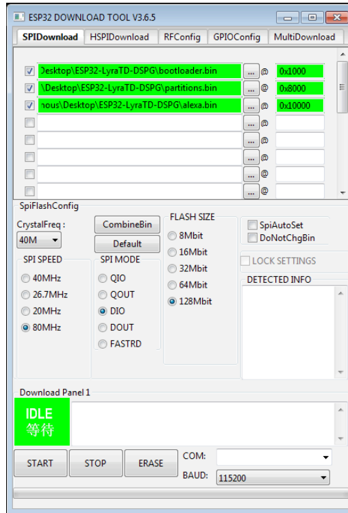
Figure 2-3. Flashing Configuration
