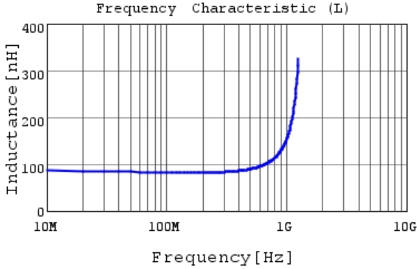
LQG15WH82NJ02 L
