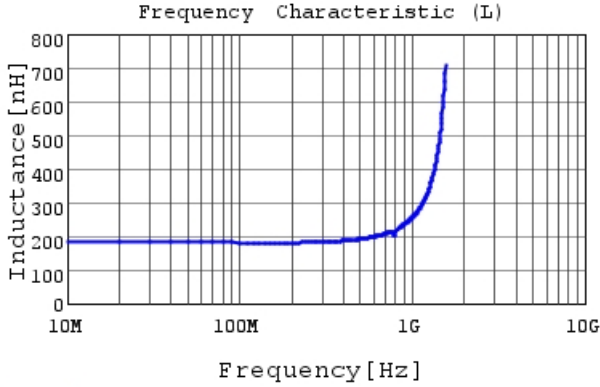
LQW15AWR18H80 L
