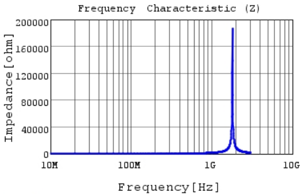
LQW15AWR18H80 |Z|
