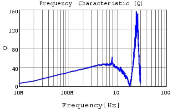
LQW15AWR18H80 Q
