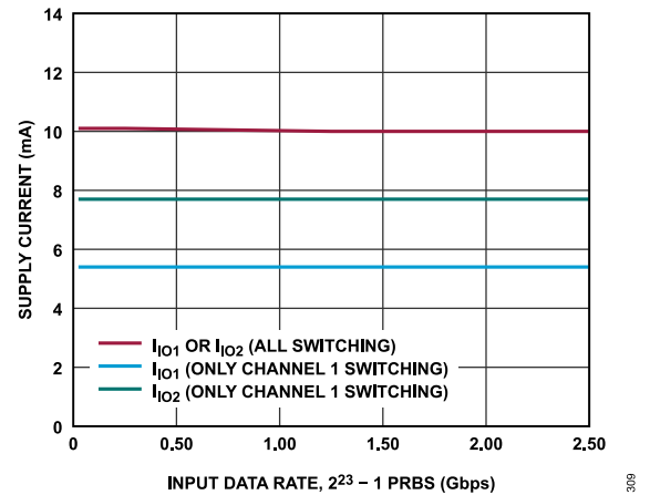
Figure 12. V_{I01} and V_{I02} Supply Current vs. Input Data Rate, 2^{23} - 1 PRBS for the ADN4622
