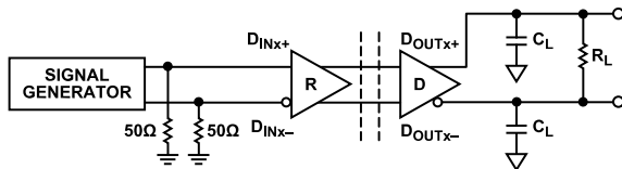
Figure 38. Voltage Definitions
