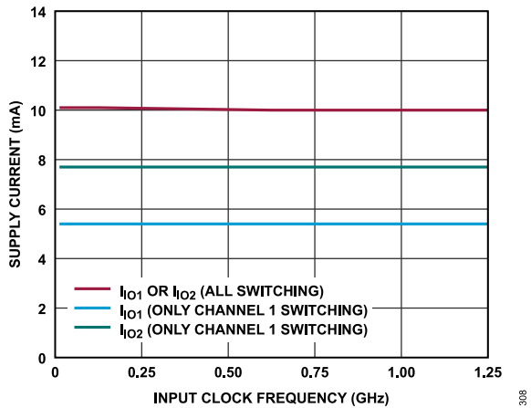
Figure 9. V_{I01} and V_{I02} Supply Current vs. Input Clock Frequency for the ADN4622
