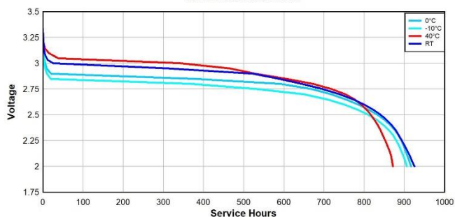
Temperature Discharge 15K Ohm Continuous to 2.0V
