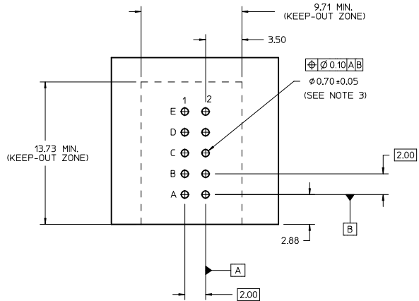
RECOMMENDED PCB LAYOUT AND KEEP-OUT ZONE
