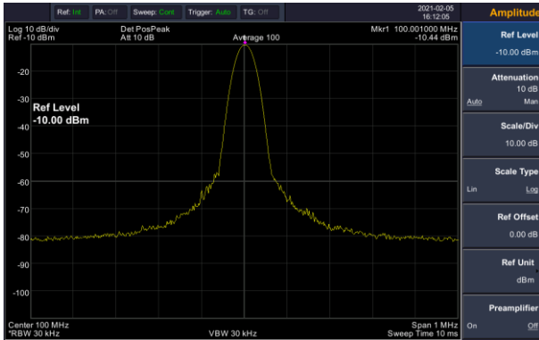
Figure 3-10 Set reference level
