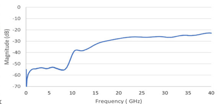
Series Return Loss (S11)
