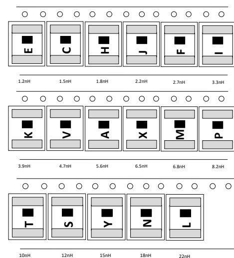
ACCU-L 0805
