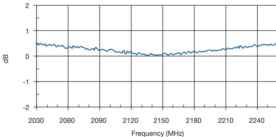
Amplitude Balance
