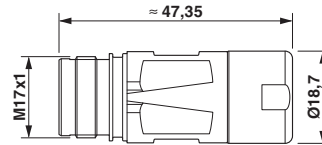
Dimensional drawing
