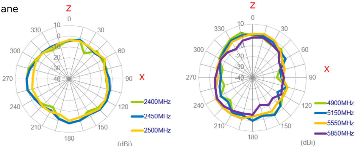
YZ Plane
