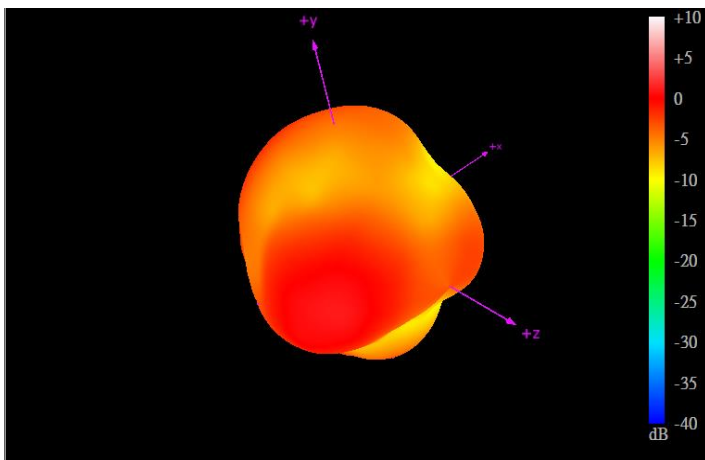
1575.42MHz
