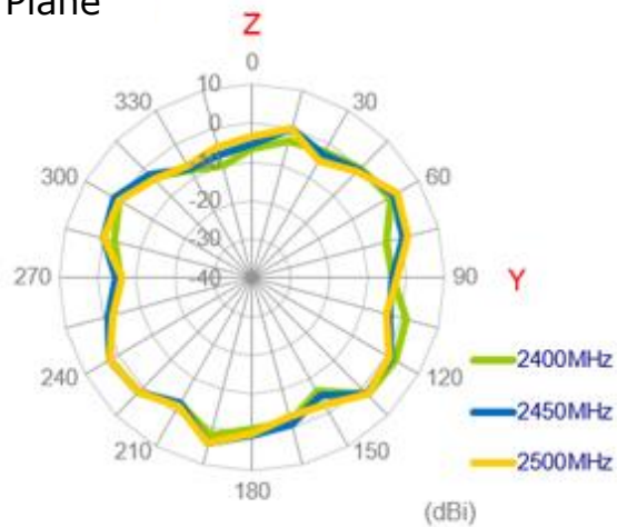
YZ Plane
