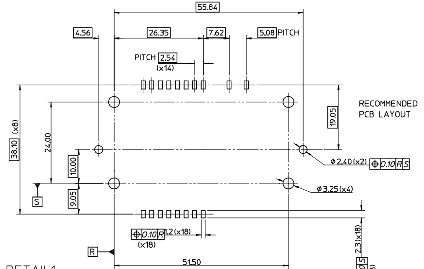
DETAIL 1
