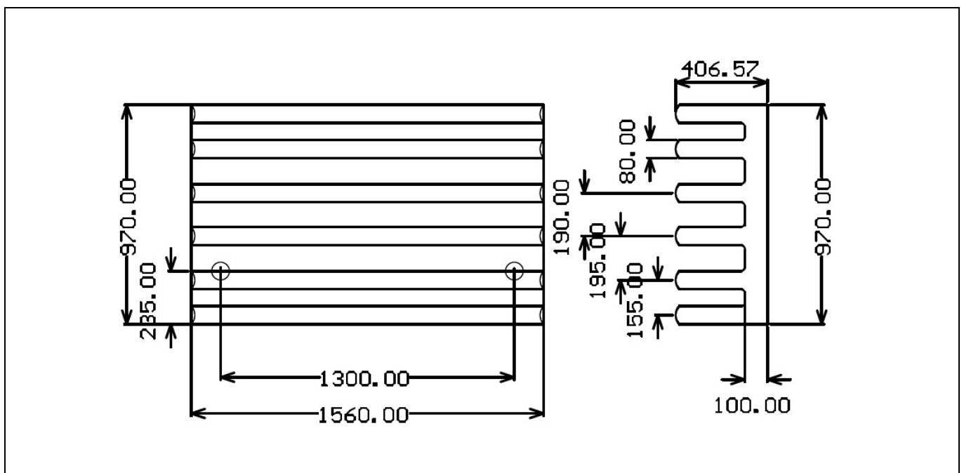
Figure 11 Heatsink dimension
