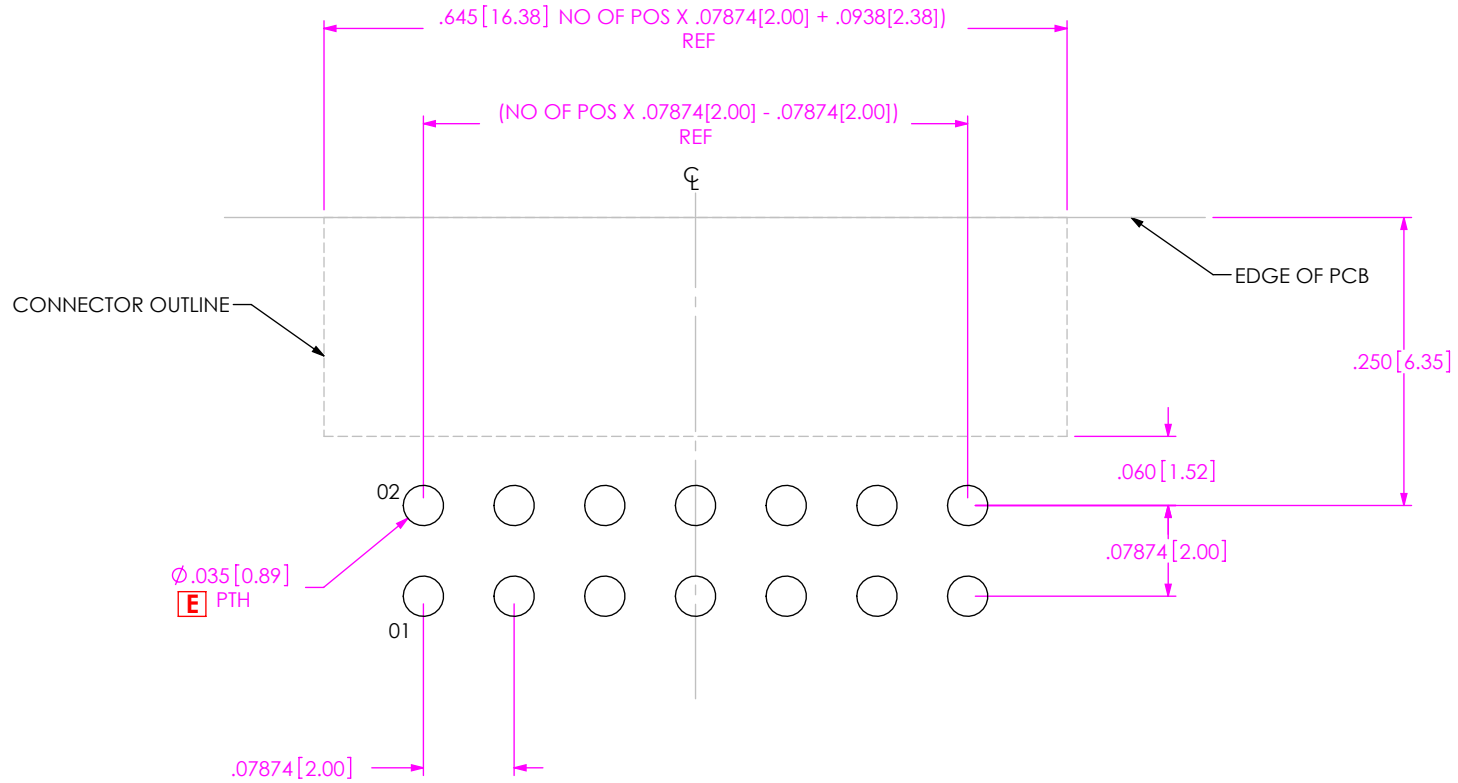
FIGURE 2 LTMM-1XX-XX-XX-D-RA-XX
