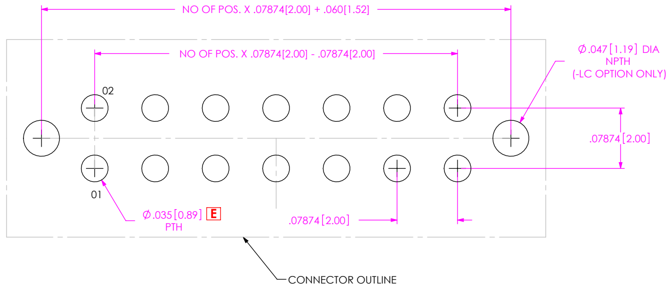
FIGURE 1 LTMM-107-XX-XX-D-LC-XX
