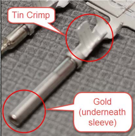
Size 20 Socket (After)
