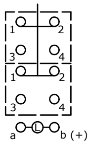
CONTACT CONFIGURATION
