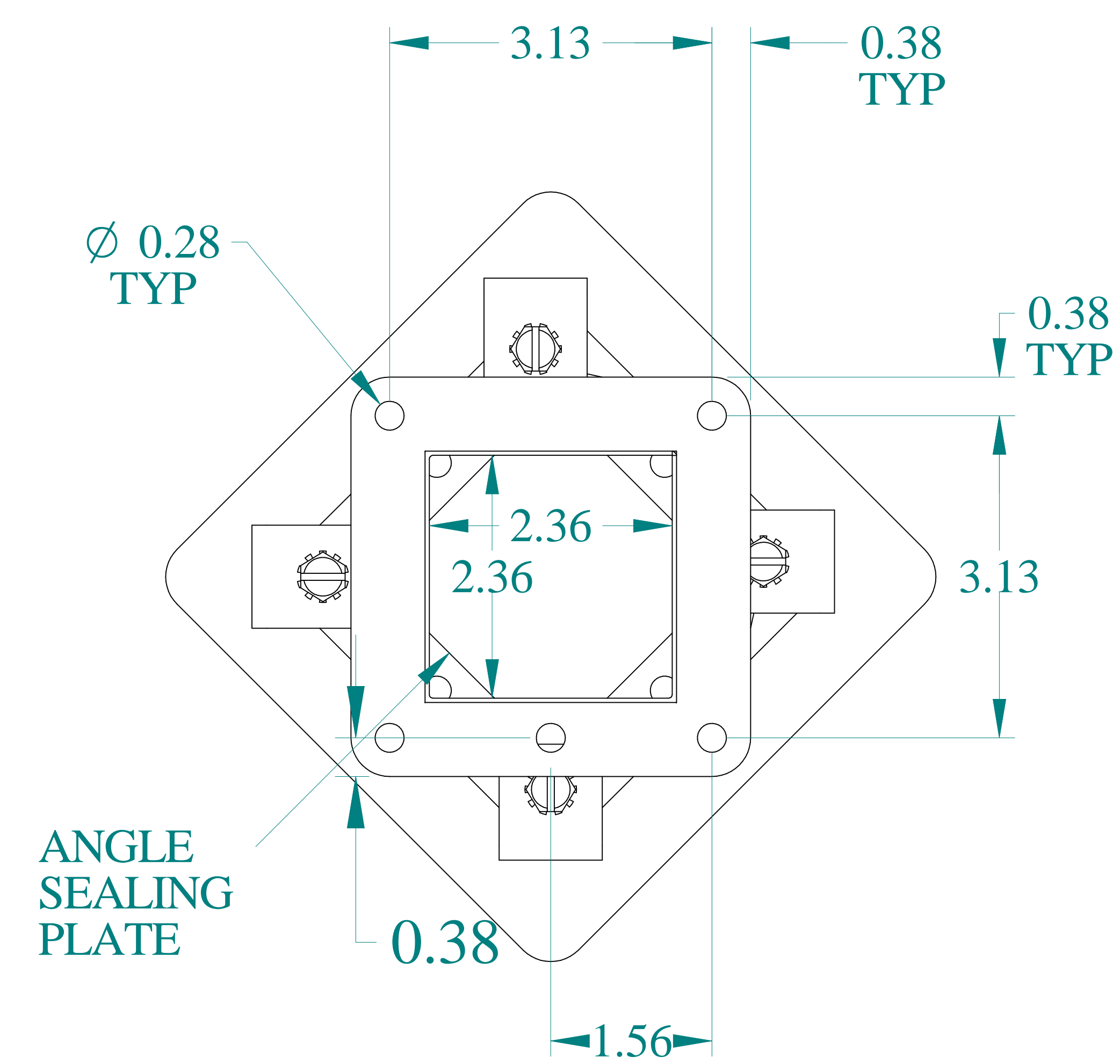
FRONT VIEW
