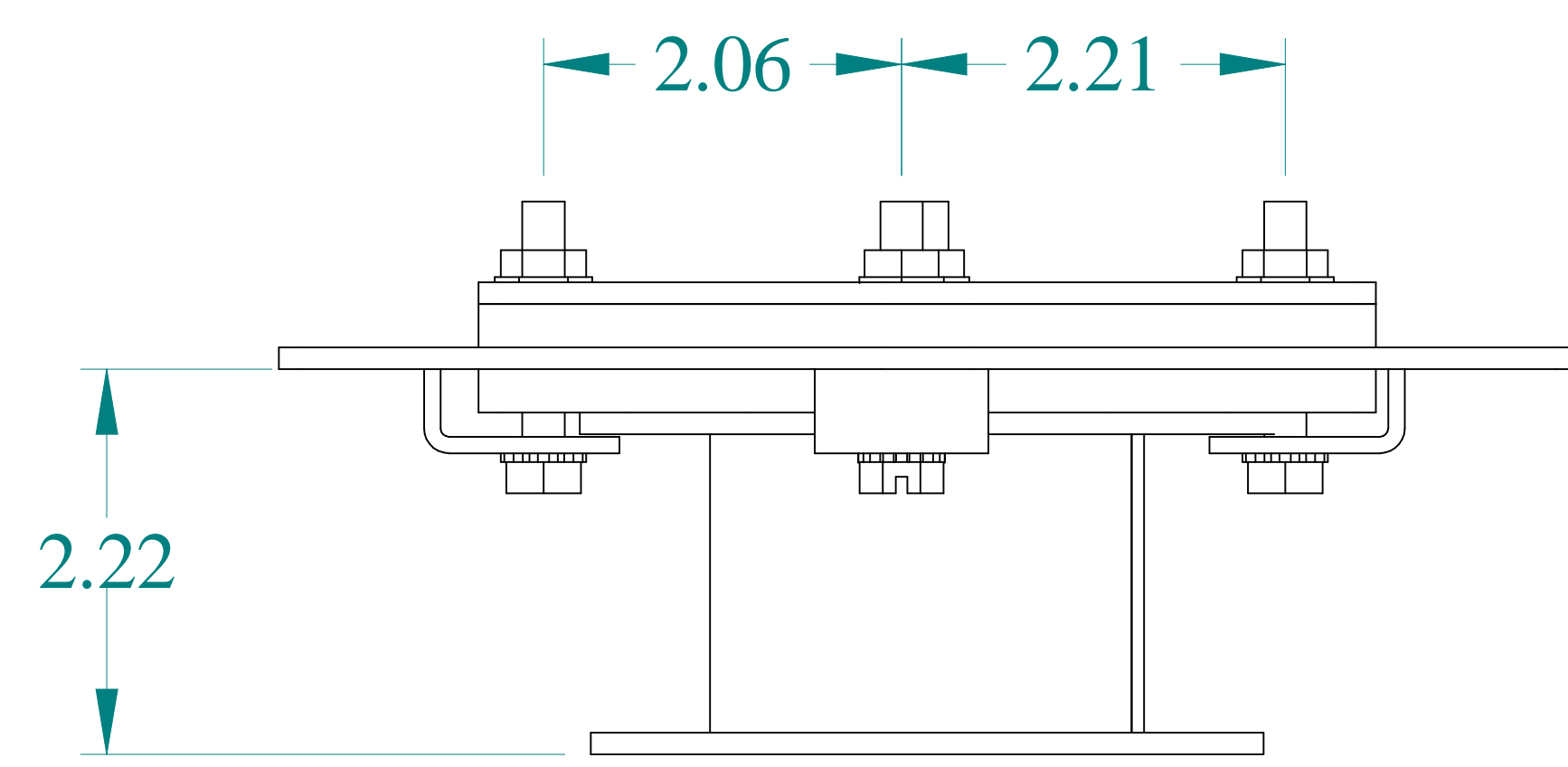
TOP VIEW
