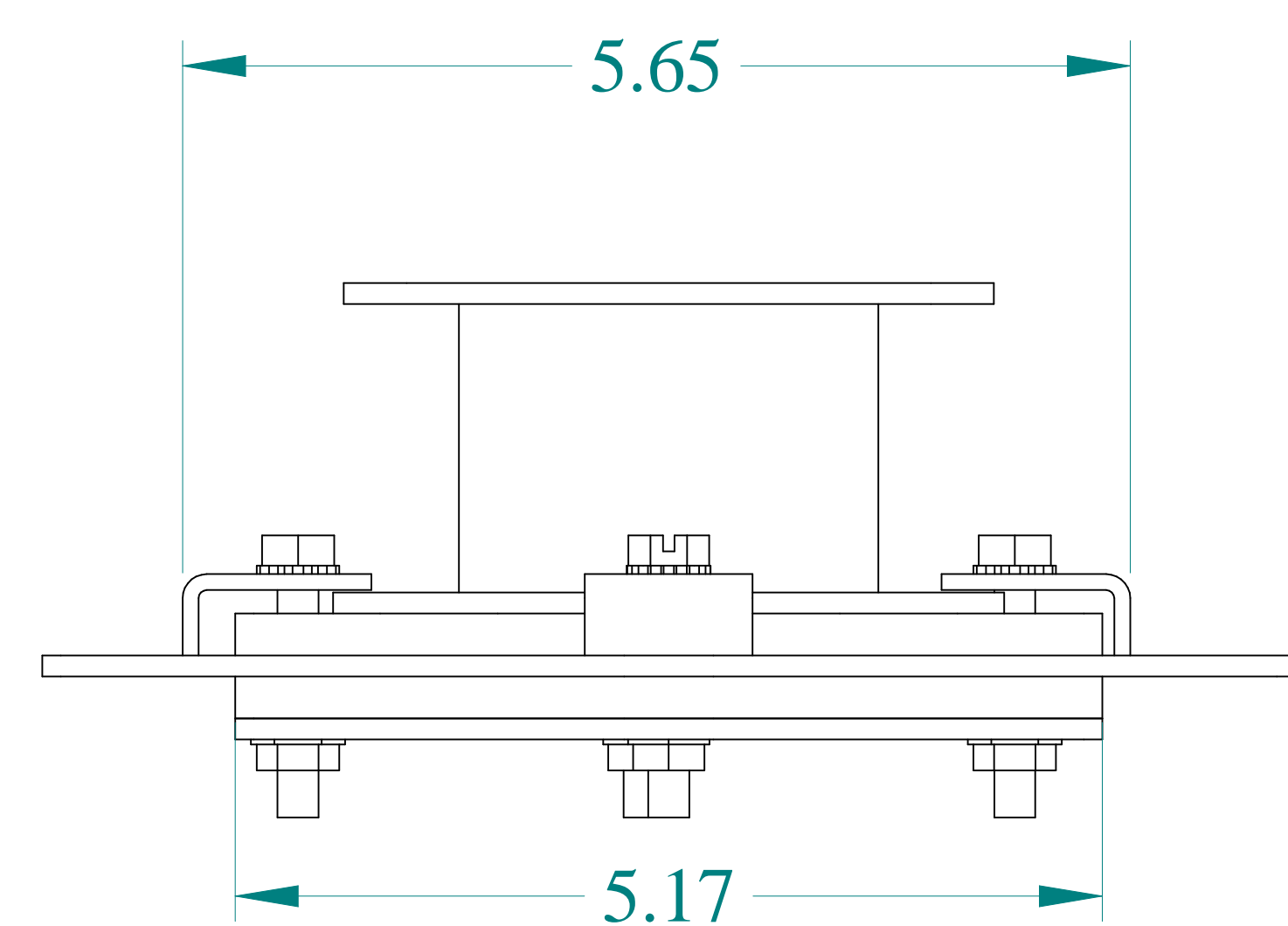
BOTTOM VIEW
