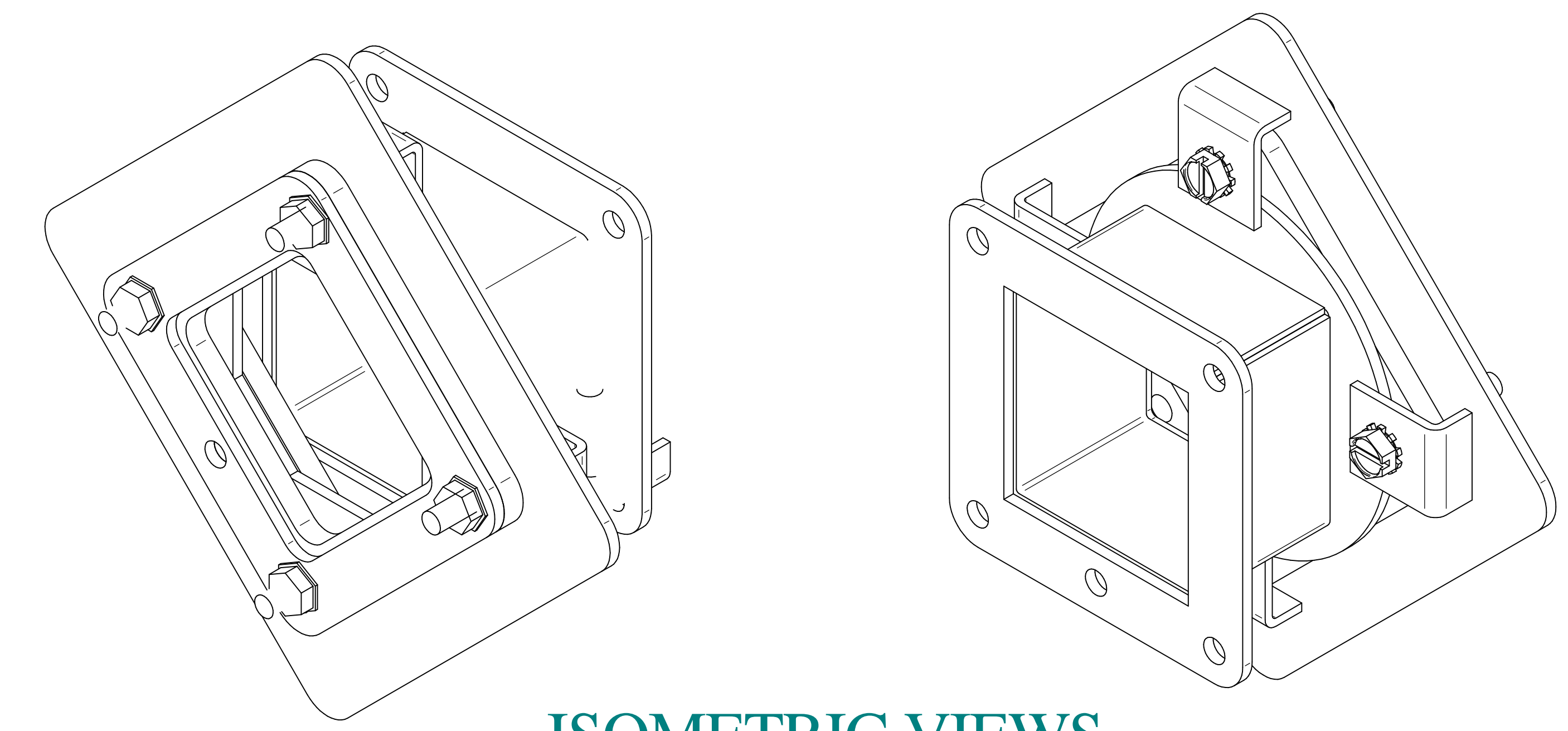
ISOMETRIC VIEWS
