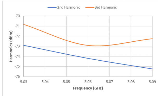
2nd & 3rd Harmonic vs. Frequency
