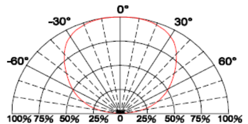
Fig.6 Directive Radiation
