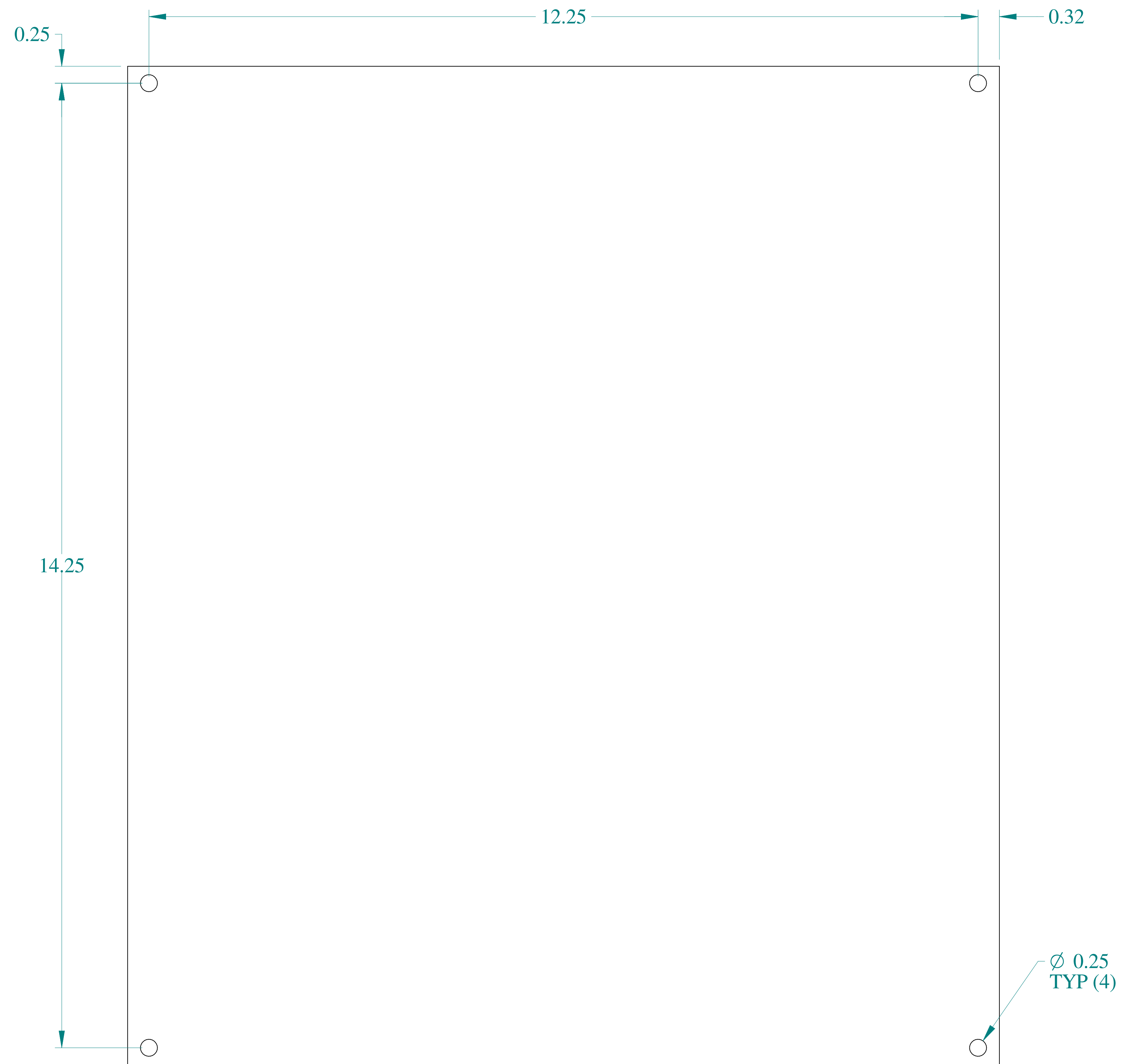
FRONT VIEW
