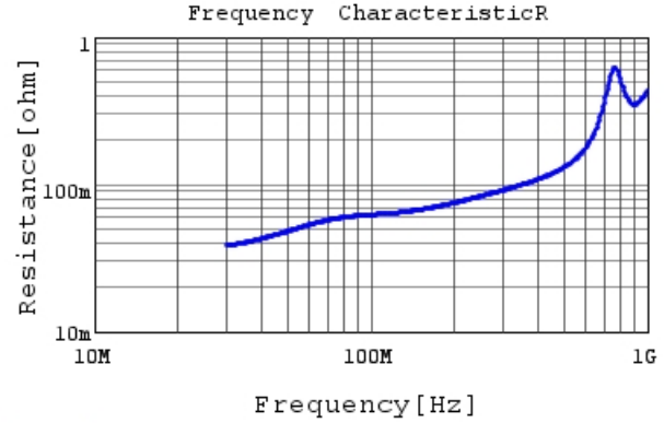
RDE5C2E471J1K1H03B R DC0V, 25degC
