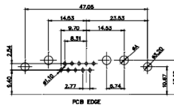
13W3 Female
