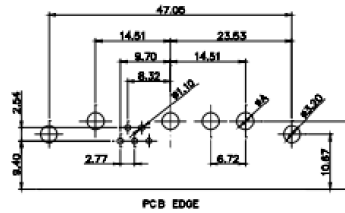
9W4 Female
