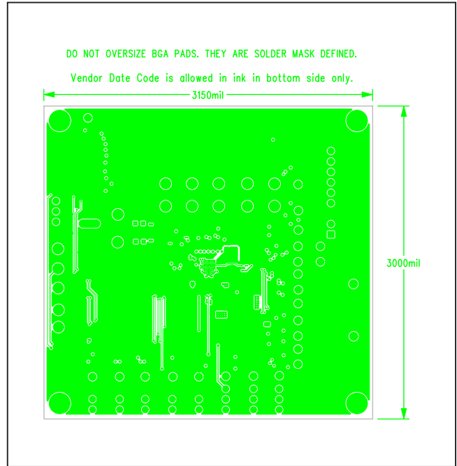
MAX77863 EV Kit PCB Layout—Layer 2 Route + GND
