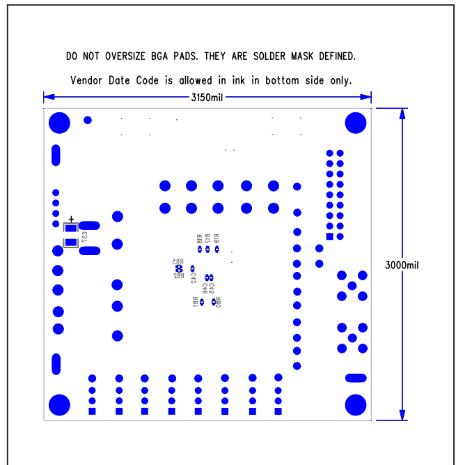
MAX77863 EV Kit PCB Layout—Bottom Silkscreen
