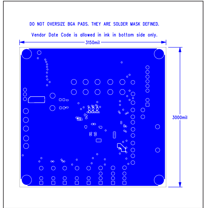
MAX77863 EV Kit PCB Layout—Bottom Layer
