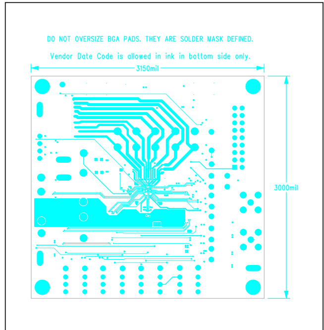
MAX77863 EV Kit PCB Layout—Layer 3 Routing
