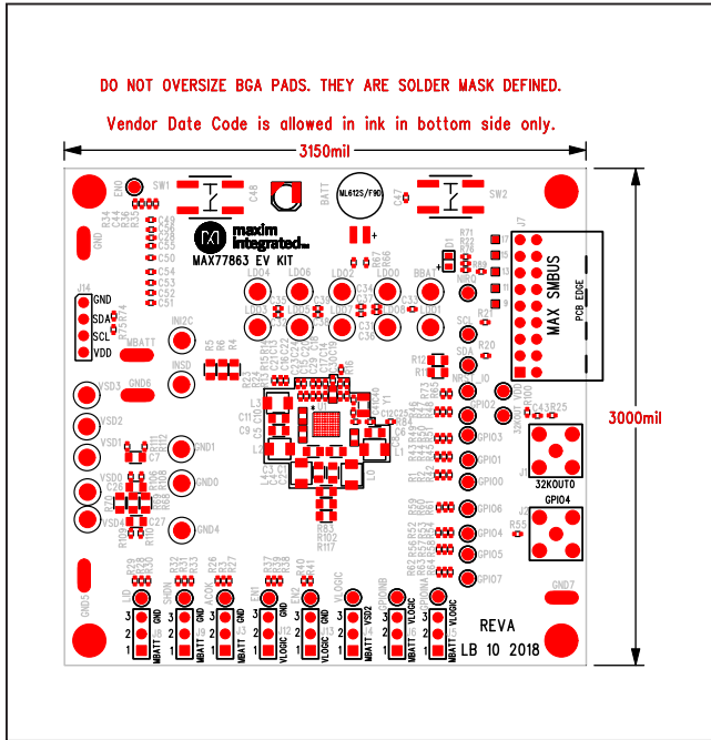
MAX77863 EV Kit Component Placement Guide—Top Silkscreen
