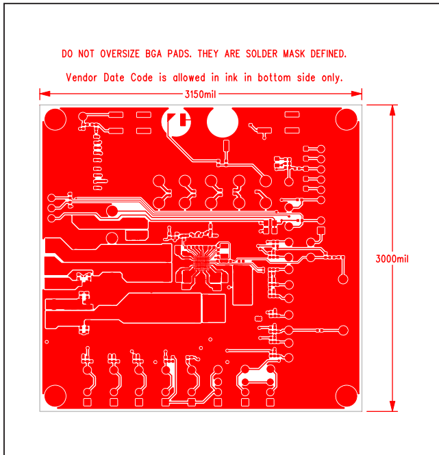
MAX77863 EV Kit PCB Layout—Top Layer
