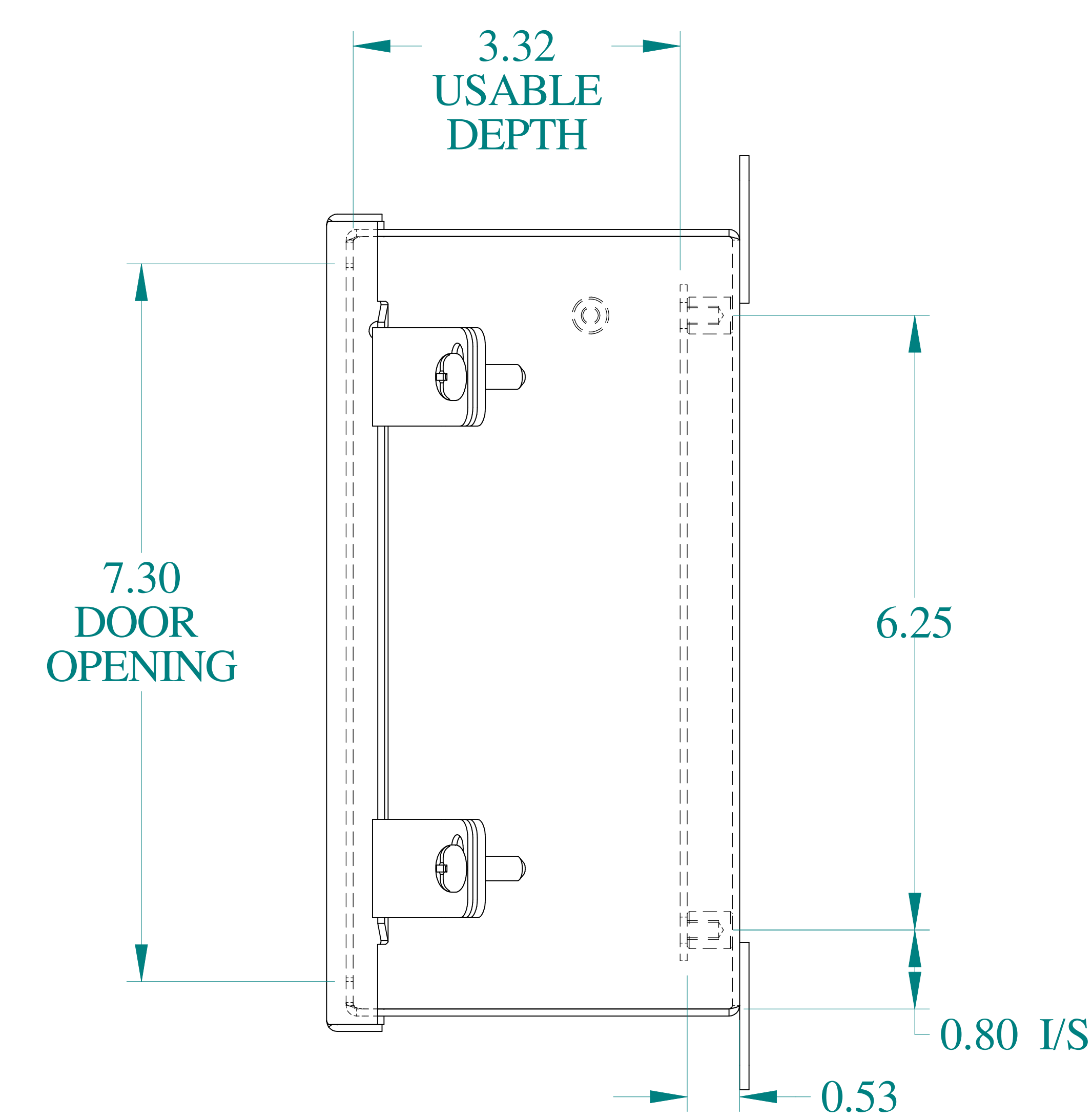
SIDE VIEW
