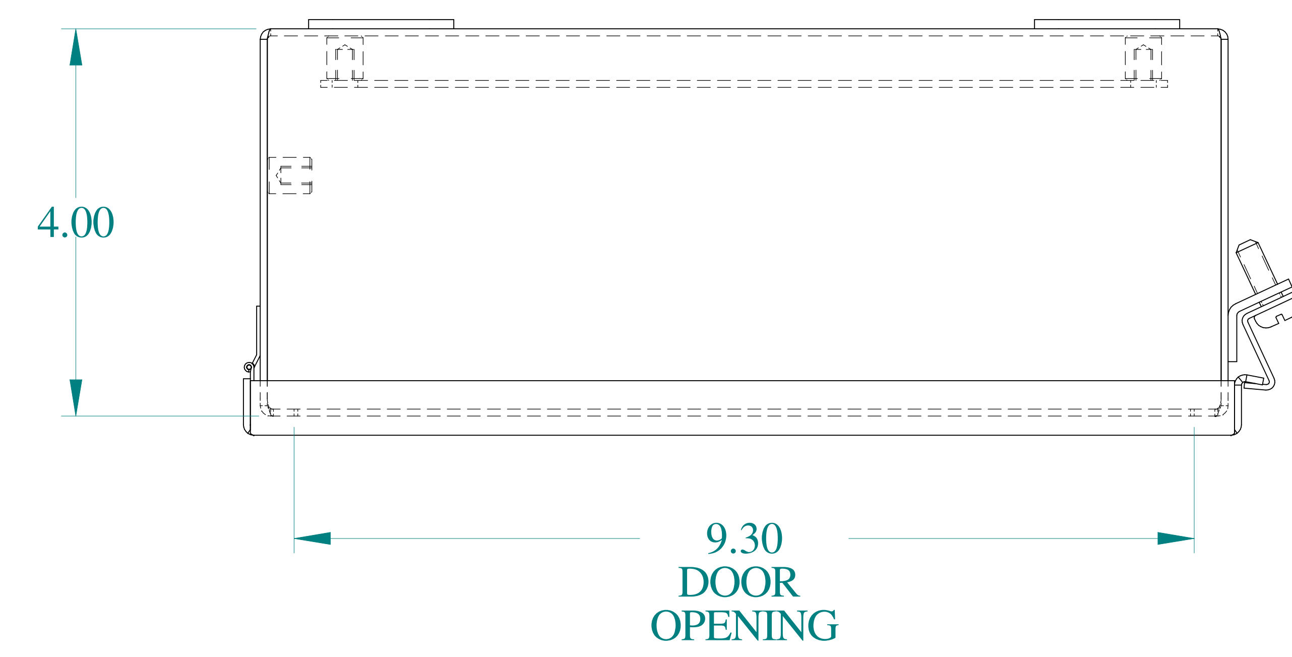
TOP VIEW
