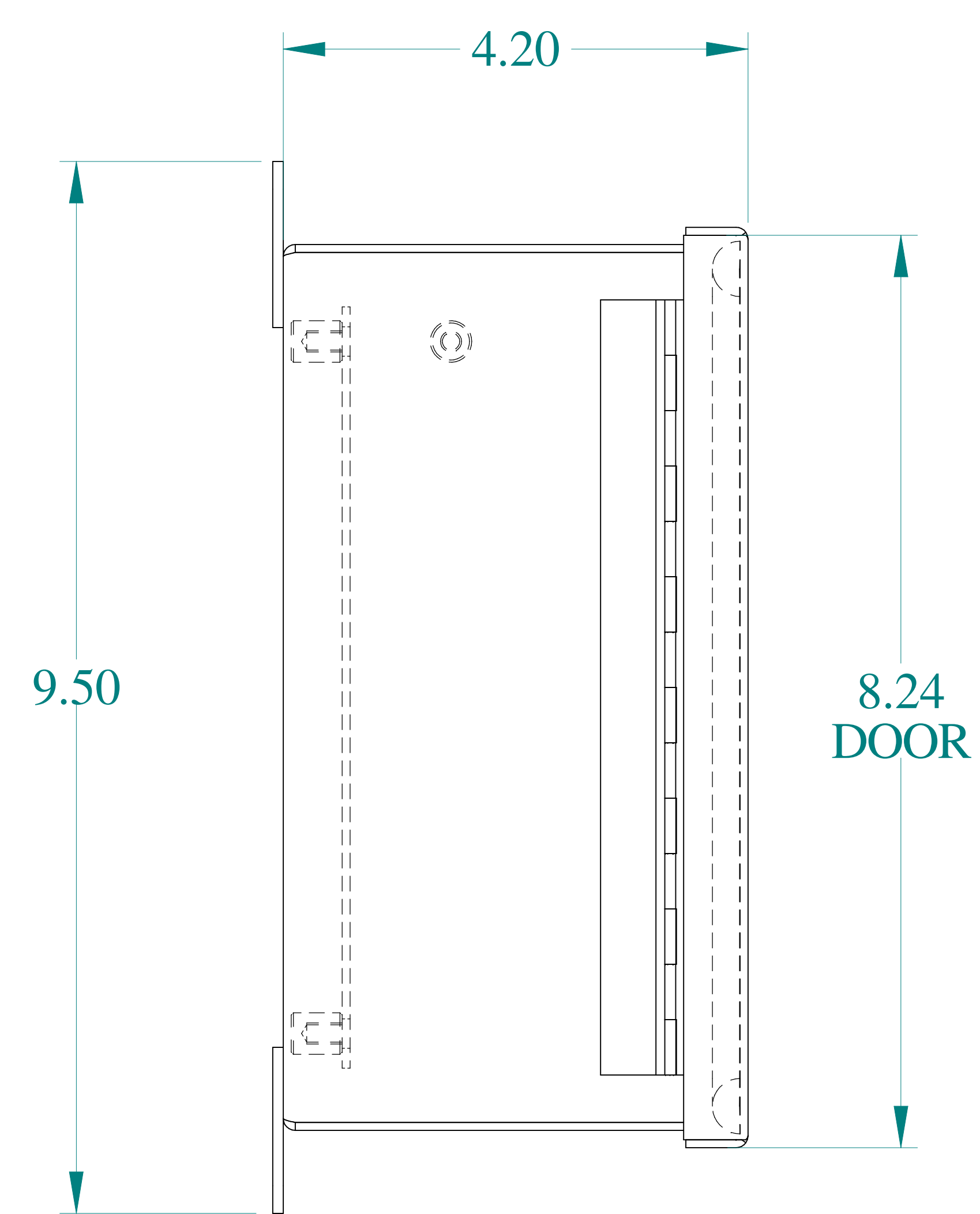
SIDE VIEW
