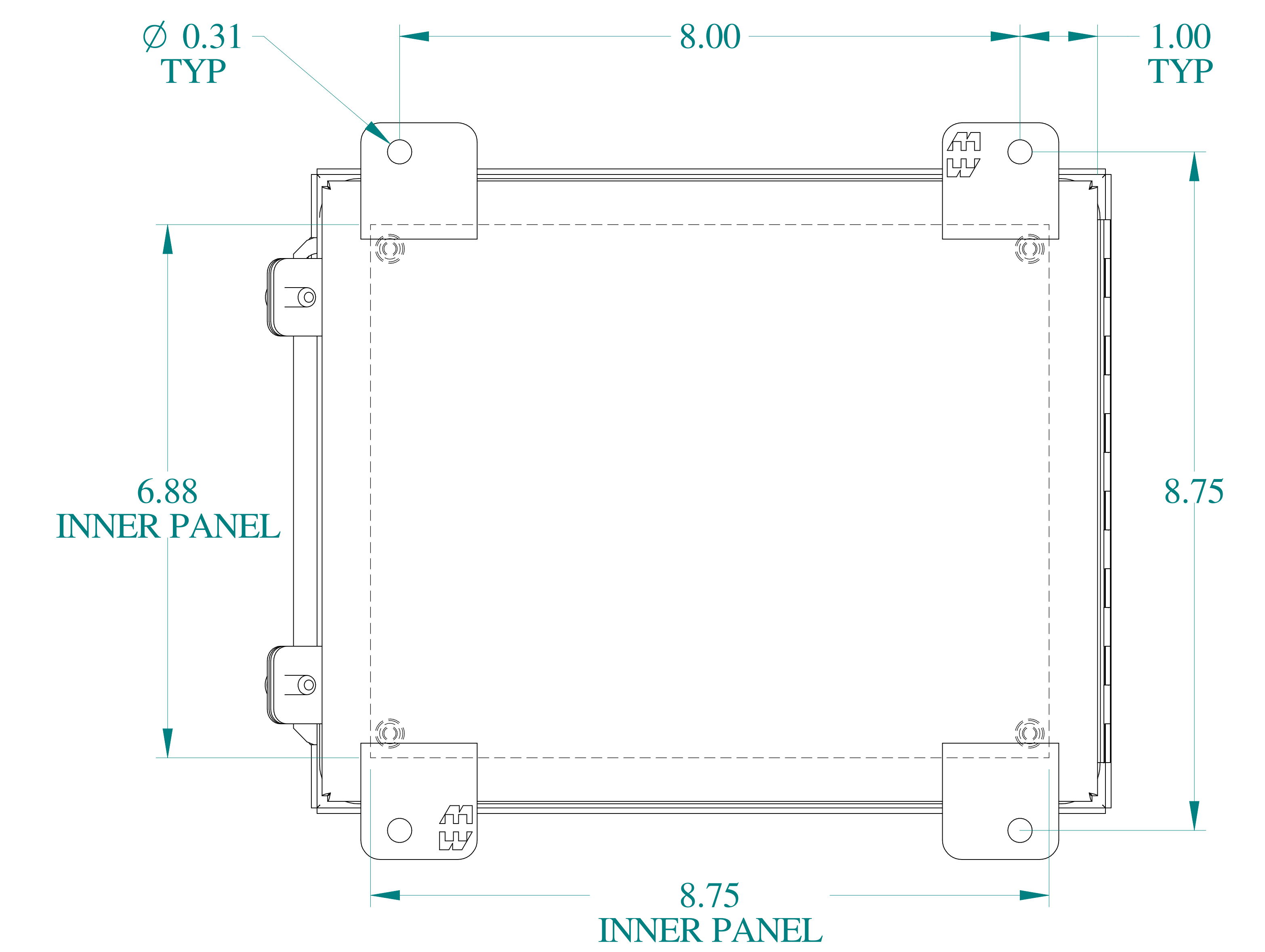
BACK VIEW
