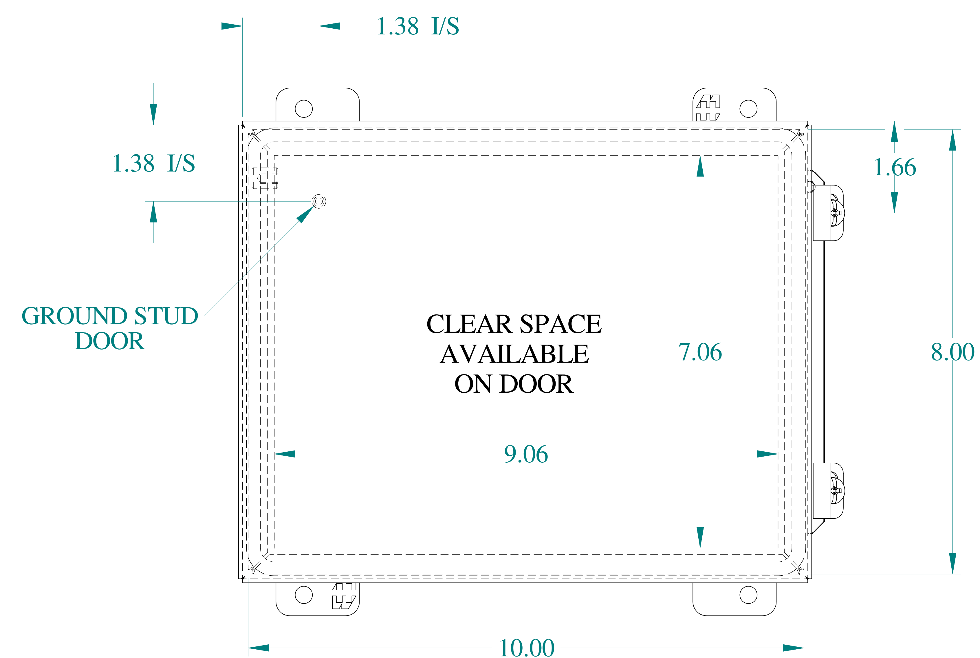
FRONT VIEW
