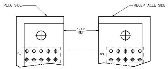
VIEW Z-Z (POWER CKTS ARE ALIGNED)
