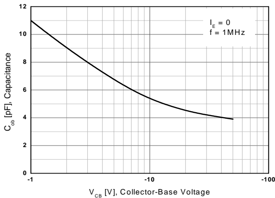
Figure 5. Output Capacitance
