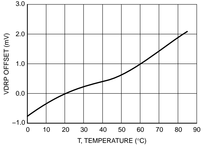
Figure 18. VDRP Offset vs. Temperature
