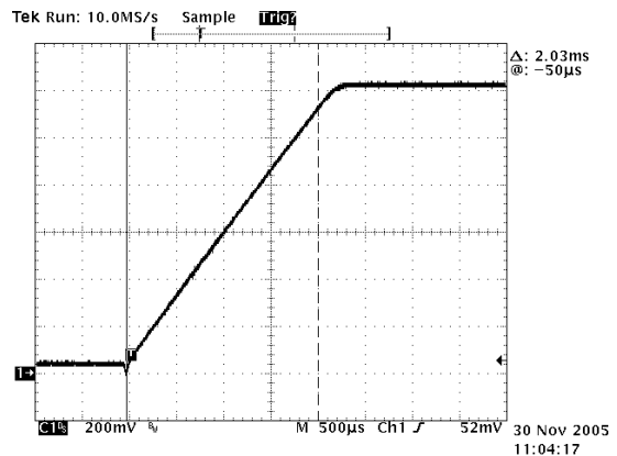
Figure 34. AMD Startup
