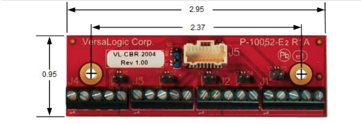
Figure 29. CBR-2004 Dimensions
