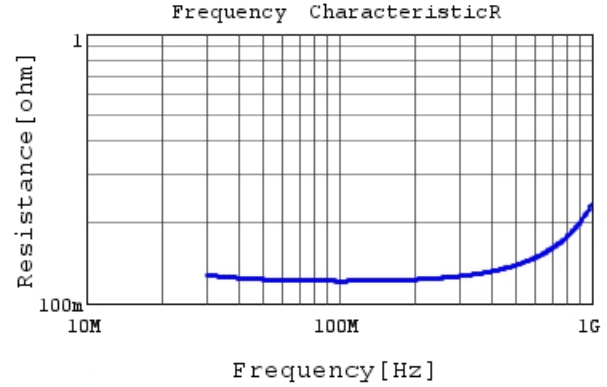
RCE5C2E181J1K1H03B R DC0V, 25degC
