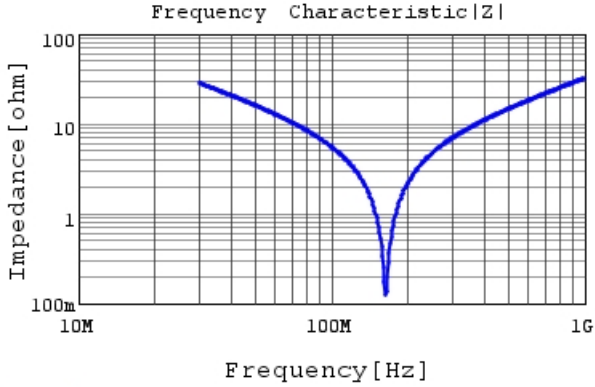
RCE5C2E181J1K1H03B |Z| DC0V, 25degC
