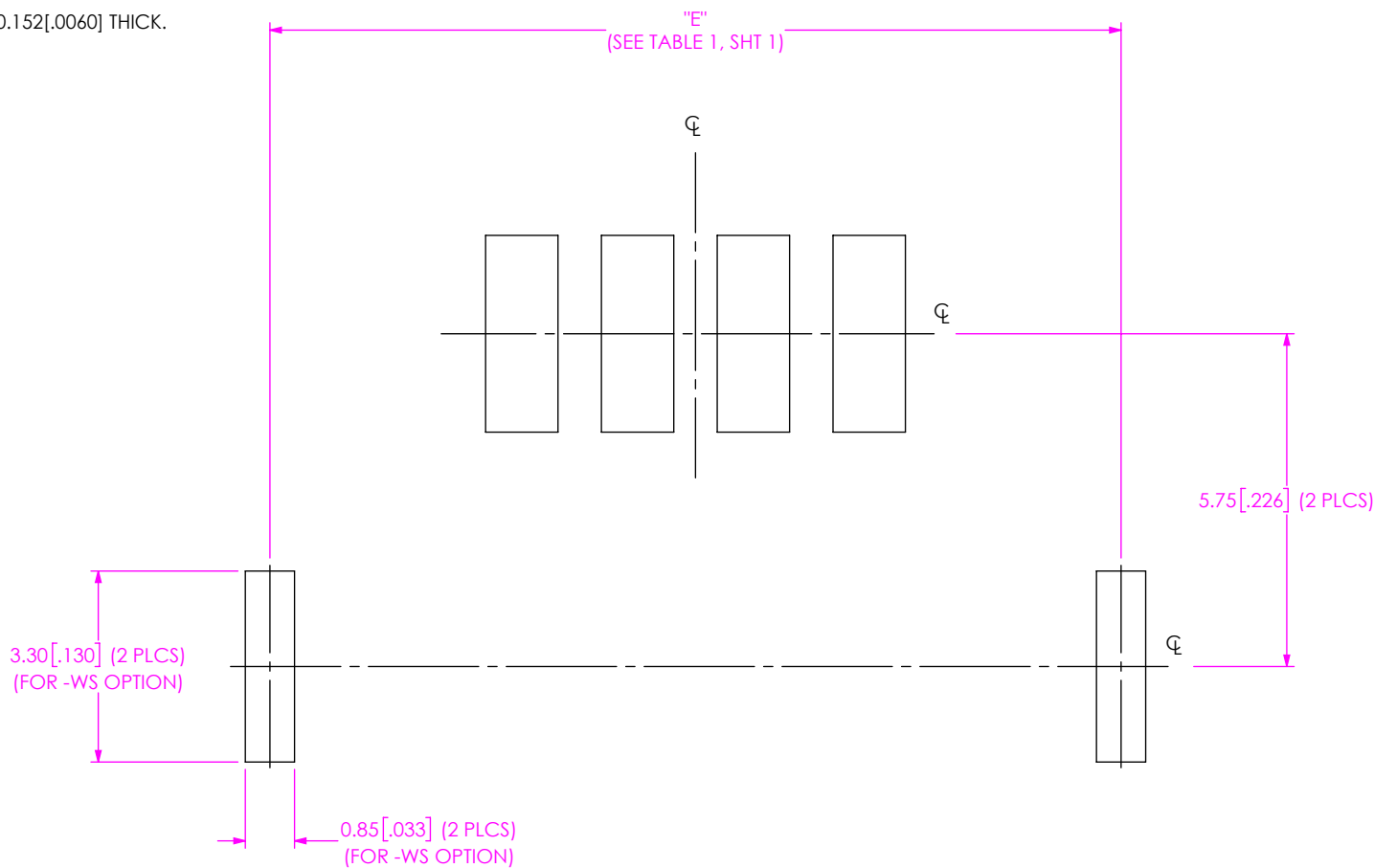
FIG 4 UMPT-04-01-XXX-RA-WS STENCIL SHOWN (DIFFERENT AS SHOWN, OTHERWISE SAME AS FIG 1 & 3)
