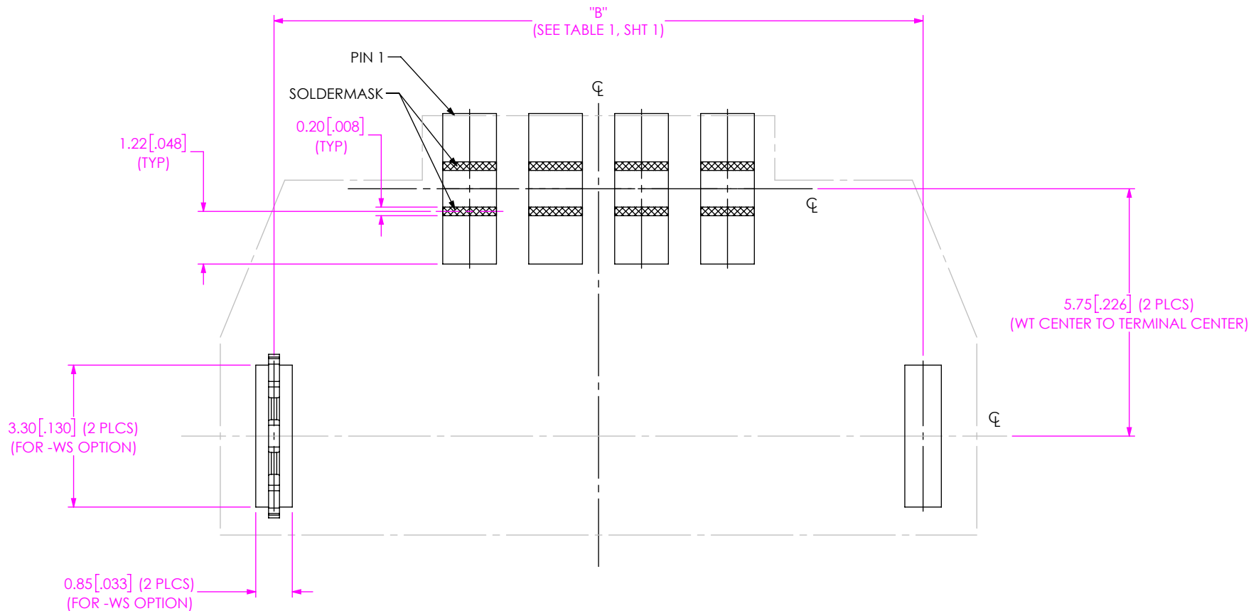
FIG 3 UMPT-04-01-XXX-RA-WS FOOTPRINT SHOWN (DIFFERENT AS SHOWN, OTHERWISE SAME AS FIG 1)
