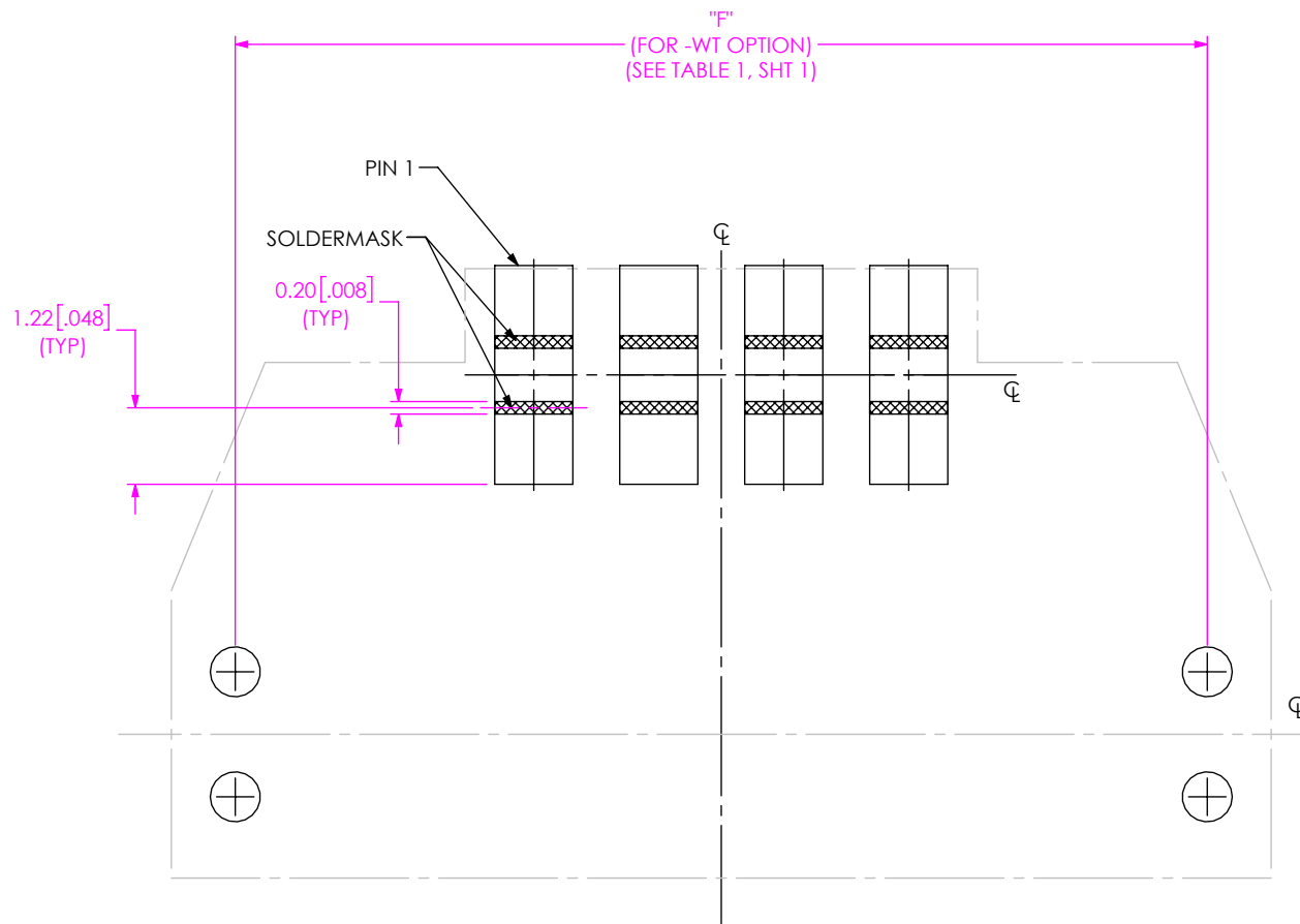
FIG 5 UMPT-04-01-XXX-RA-WT-M FOOTPRINT SHOWN (DIFFERENT AS SHOWN, OTHERWISE SAME AS FIG 1)
