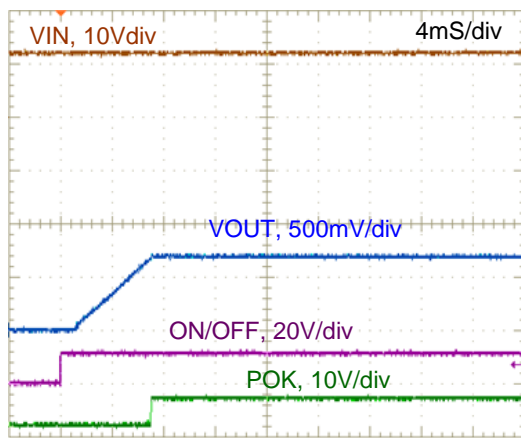
Figure 31. On/Off Enable wave form @+25°C (VIN=12V, VOUT=0.7V, IOUT=6A)
