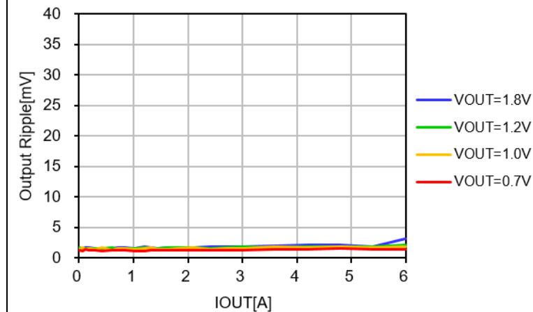
Figure 6. Output Ripple vs. Load Current and Output Voltage (COU=200μF, ScopeBW=20MHz)
