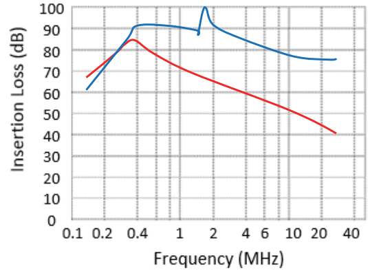
TB1-10A080H
