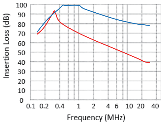
TB1-06A0D0H
