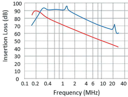
TB1-06A080H
