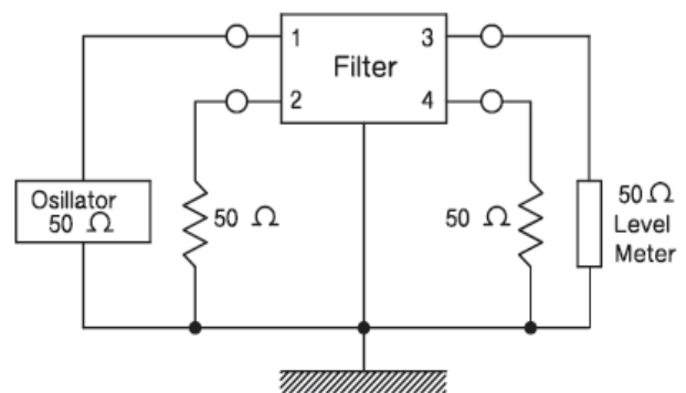
Differential mode
