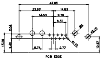
13W3 Male
