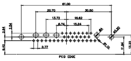
36W4 Male
