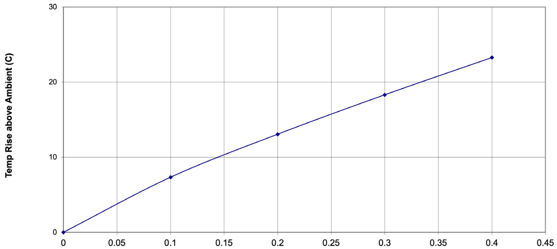
PA5190.XXHLT Temp Rise vs Power Dissipation
