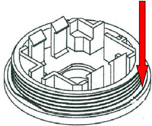
New drawing (Add step inside the bottom housing)
