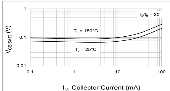
Fig.2 Collector-Emitter Saturation Voltage
